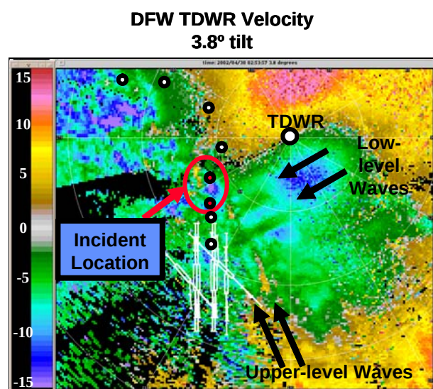
Figure 5. A Doppler velocity image from the DFW TDWR at the time of the intersecting buoyancy waves encounter on 30 April 2002. The arrows illustrate the locations of the two sets of BW waves. Dots represent the flight path of the MD-80 and the red dots denote the location where the aircraft encountered the severe turbulence. Scale shown in units of m/s.
