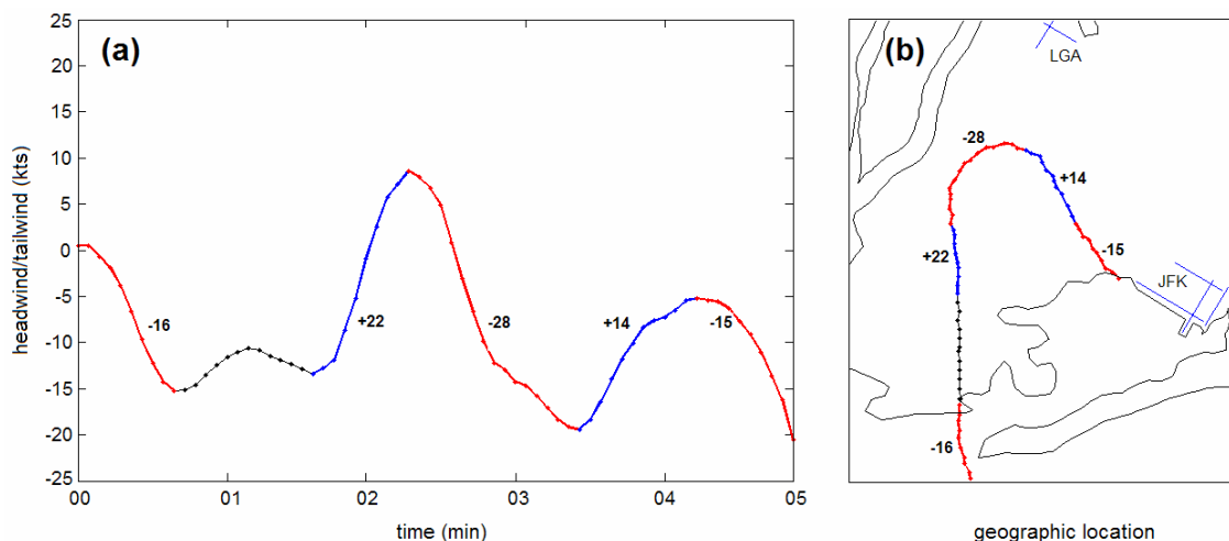
Figure 10. (a) Headwind profile of Boeing 767 on April 29, 2002. The ordinate axis indicates headwind/tailwind (kts) as positive/negative values respectively. Segments plotted in red indicate calculated potential aircraft airspeed losses exceeding -10kts; gains greater than 10 kts are plotted in blue. Calculated values at each loss/gain segment (kts) are labeled next to the curve. (b) Planar view showing geographic location of loss/gain segments for reference to Figure 10b.
