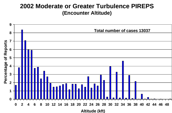
Figure 2. An altitude distribution of turbulence pilot reports over the 2002 calendar year over the Corridor Integrated Weather System domain. The PIREPs data set was provided by the National Center for Atmospheric Research (NCAR).
