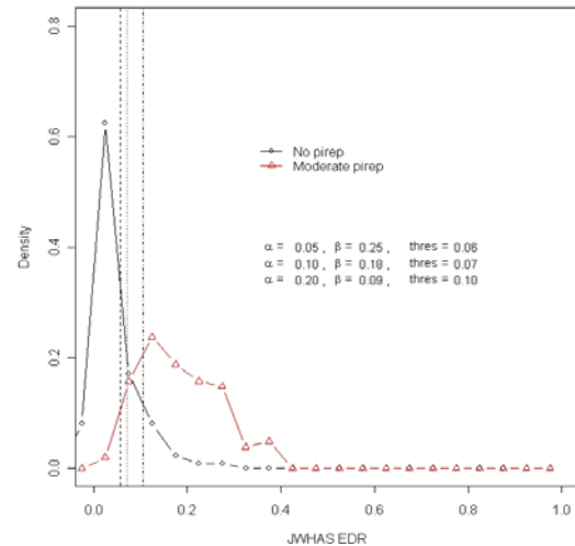
Figure 2: Discrimination plot of JWHAS nowcast EDR values for PIREPs of "No turbulence" vs. "Moderate or severe turbulence".
