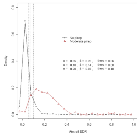
Figure 3: Discrimination plot of aircraft measured ZEDR values for PIREPs of "No turbulence" vs. "Moderate or severe turbulence".
