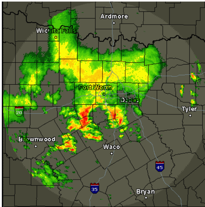
Figure 7. KFWs base reflectivity image at 21:52 UTC, May 27, 2002.
