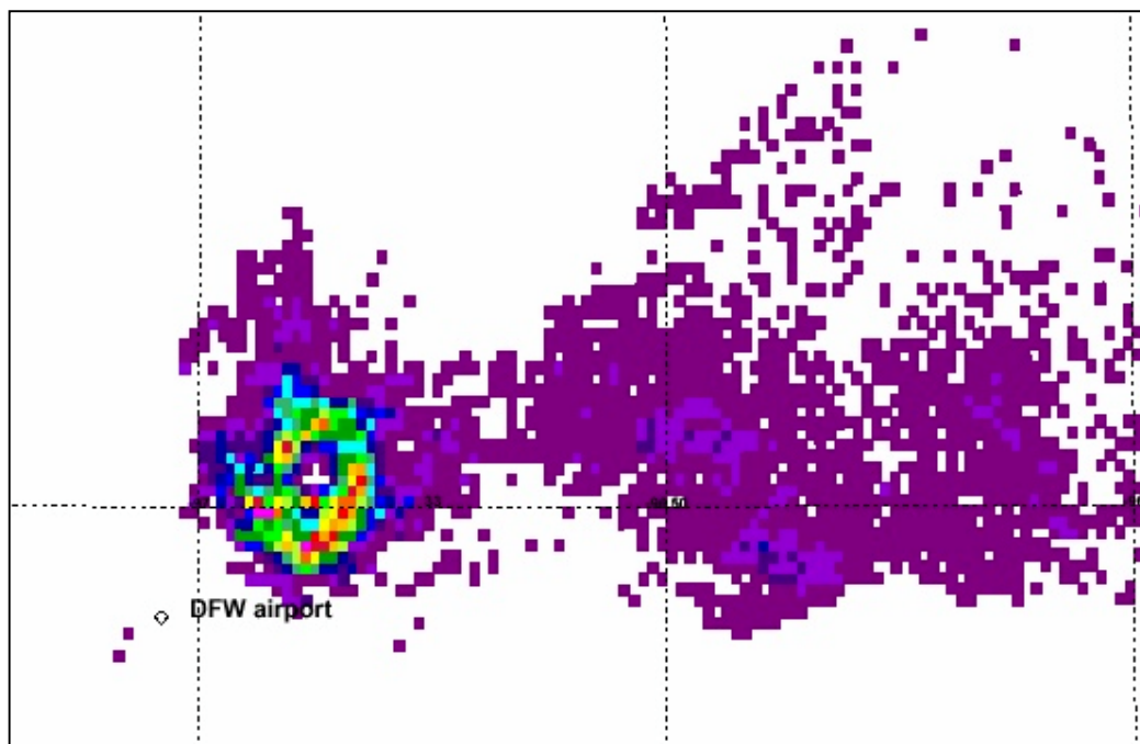
Figure 1. VHF source density ( \text{src}/\text{km}^2 ) on 1\text{X}1\text{ km}^2 grid for 04:04-04:07 UTC on April 6, 2003. Each color change represents an additional 10\text{ src}/\text{km}^2 .
