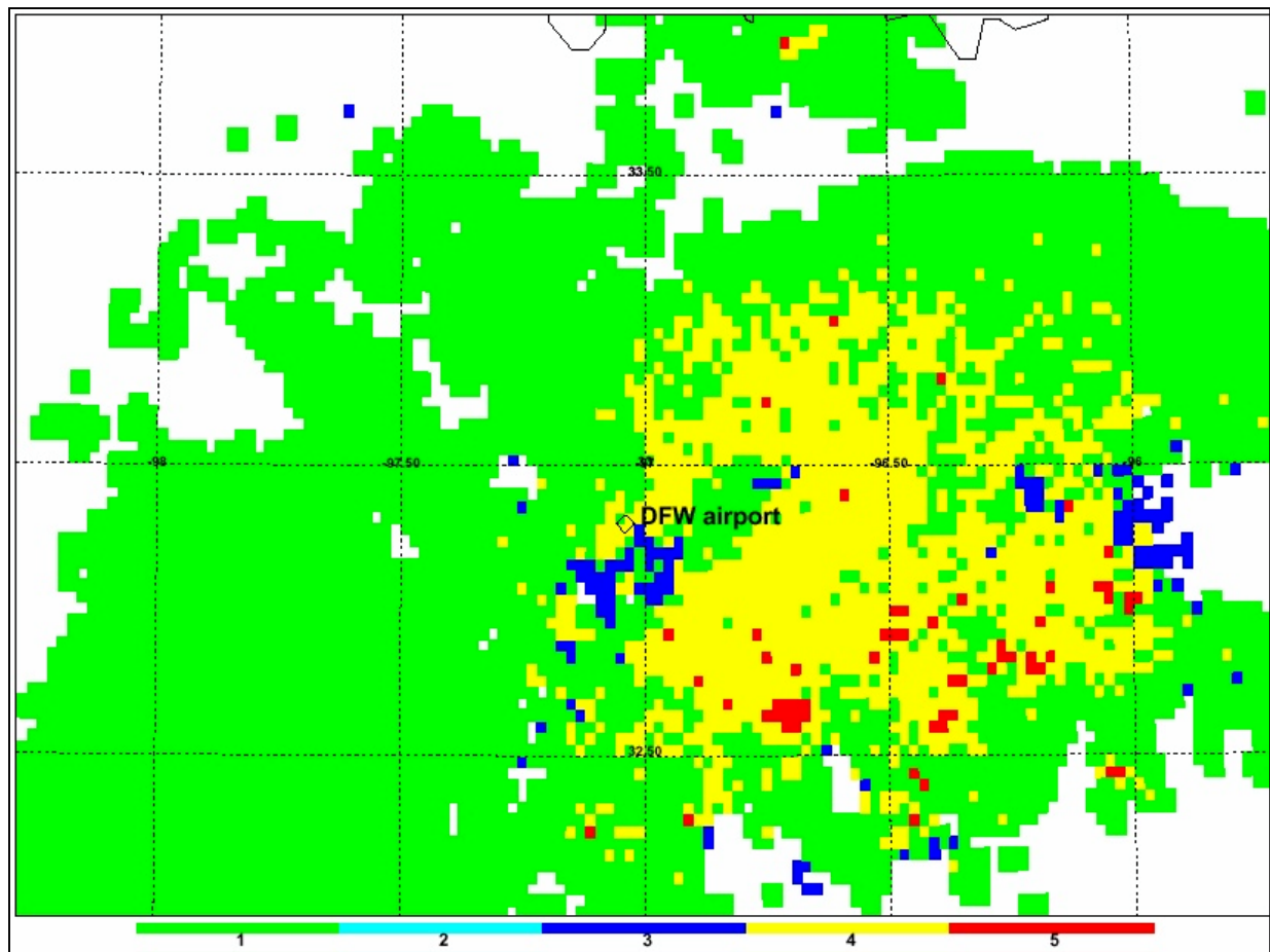
Figure 6. Prototype warning graphic based on combination of radar base reflectivity, in-cloud lightning, and CG flash information. See text for discussion of five color-coded categories.
