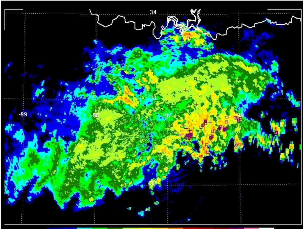
Figure 4. KFWS base reflectivity at 15:12 UTC on August 17, 2001, with CG flashes between 15:05-15:15 plotted with purple symbols (square = negative, plus sign = positive).
