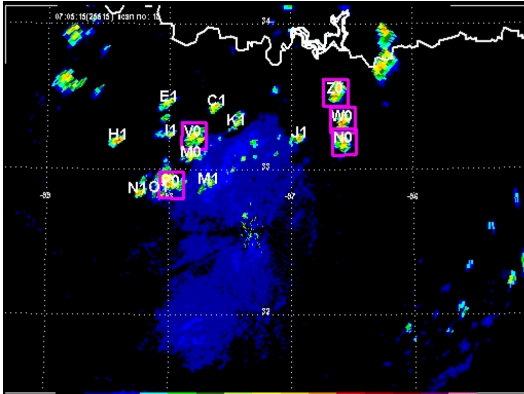
Figure 3. KFWS base reflectivity at 07:05 UTC on June 30, 2001, with cell identifiers from the SCIT algorithm shown in white. Cells with lightning are surrounded by pink boxes.
