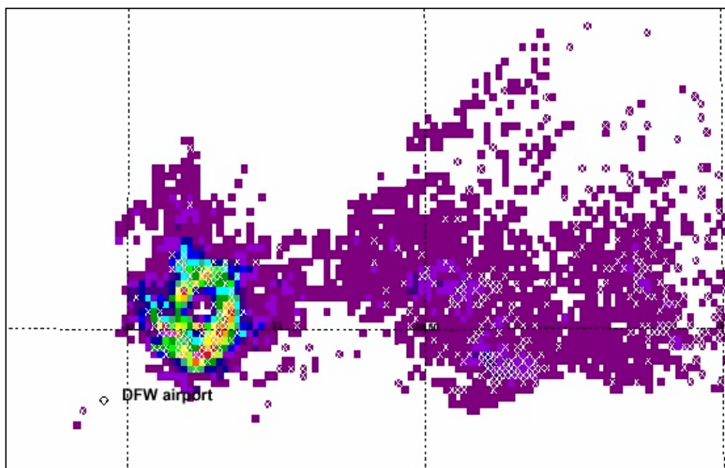
Figure 2. As in Fig. 1 but with white Xs through grid cells that include flash initiation locations.
