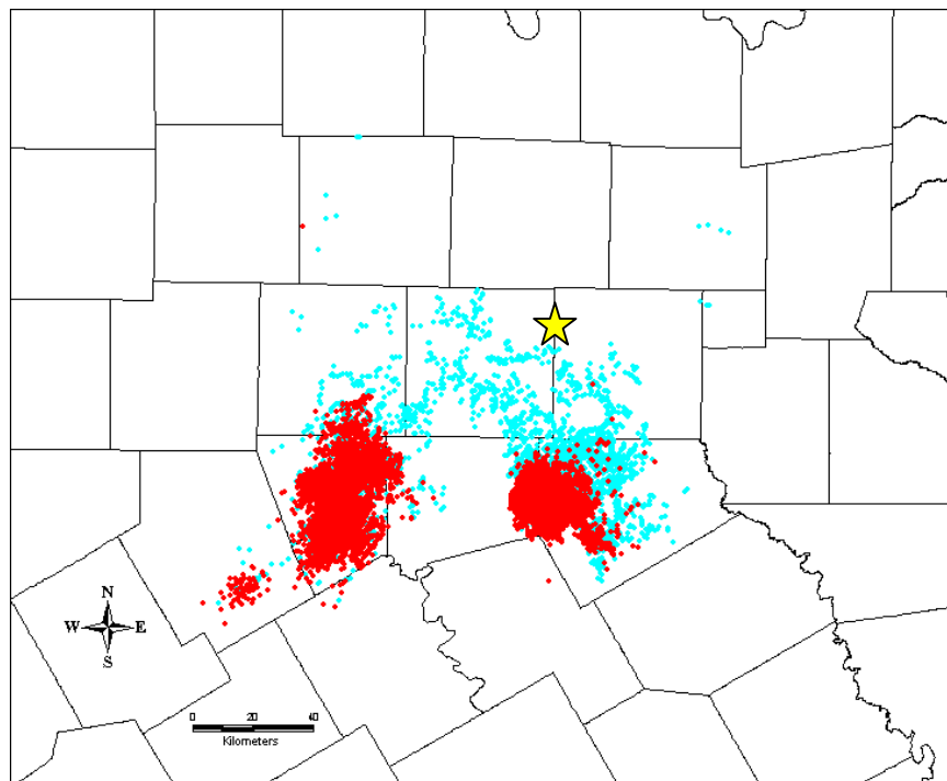
Figure 8. LDAR II sources corresponding to radar data in Fig. 7. Red: above 10 km MSL altitude; cyan: below 10 km MSL. Position of DFW airport indicated by star. County boundaries included (c.f. Fig. 7).
