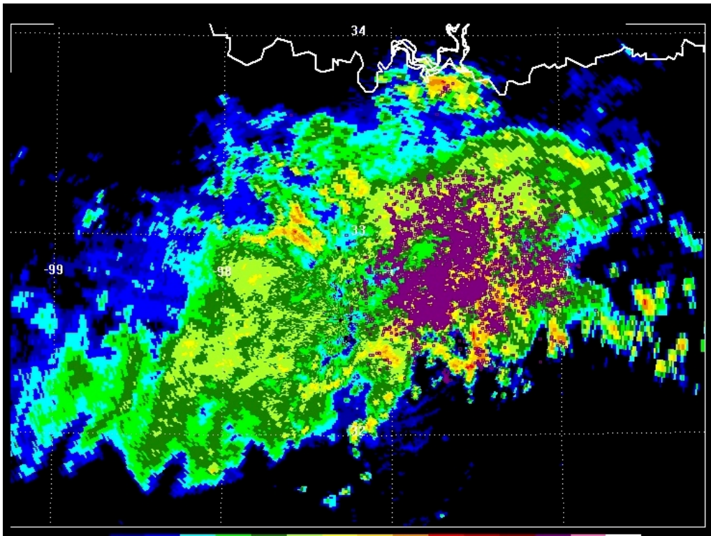
Figure 5. KFWS base reflectivity at 15:12 UTC on August 17, 2001, with LDAR II sources between 15:05-15:15 plotted with purple symbols.
