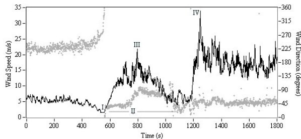
Figure 2. Wind speed (black) and direction (grey) time history of derecho. Start of event (I), IS (II), IG (III), and PG (IV) are labeled.
