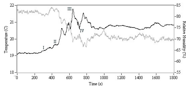
Figure 3. Fast-response temperature (black) and RH (grey) time histories of RFD. Start of event (I), IG (II), PG (III), and downburst 'eye' (IV) are labeled.
