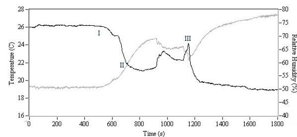
Figure 4. Fast-response temperature (black) and RH (grey) time histories of derecho. Start of event (I), IG (II), and PG (III) are labeled.
