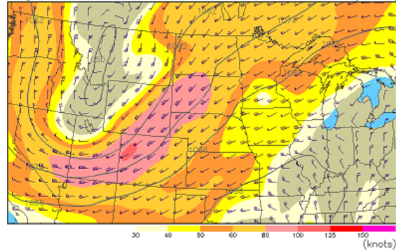
700 mb Heights (dm) / Isotachs (knots)
