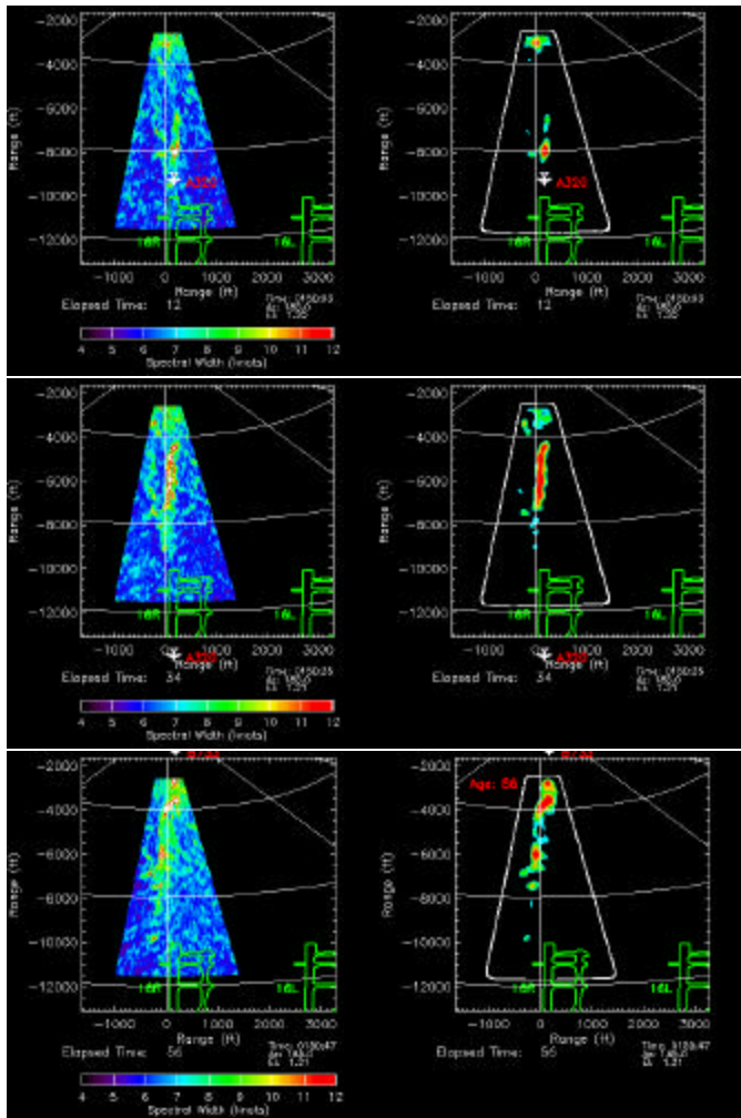
Figure 7 Sample glide slope viewing example from DEN. Snapshots from three scans are provided. Each two-panel display shows the estimated spectral width on the left and a thresholded version of the spectral width on the right. The panels are plan views of the approach corridor to runway 16R at DEN.
