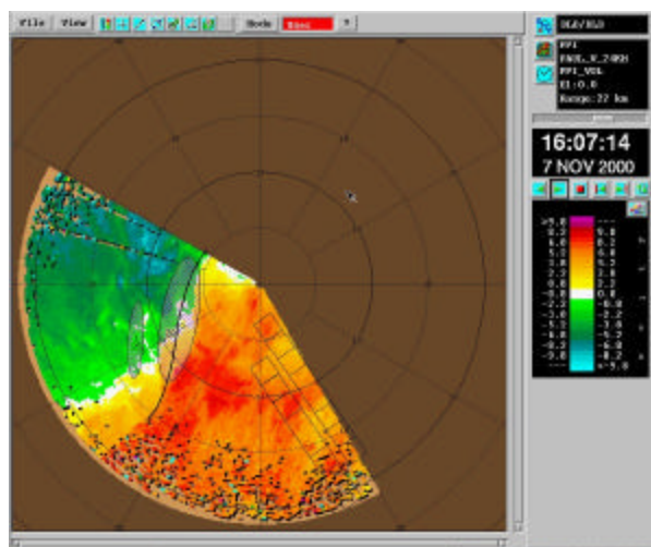
Figure 3 Sample plan position indicator (PPI) display of measured radial velocity. The velocity data is color-coded with positive velocities defined as away from the lidar. A shear line algorithm is applied to the data and icons indicate the location of the gust front relative to the airport approach and departure corridors.
