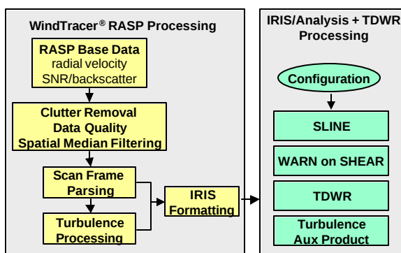
Figure 2 Block diagram of processing flow for wind hazard situation display product generation.
