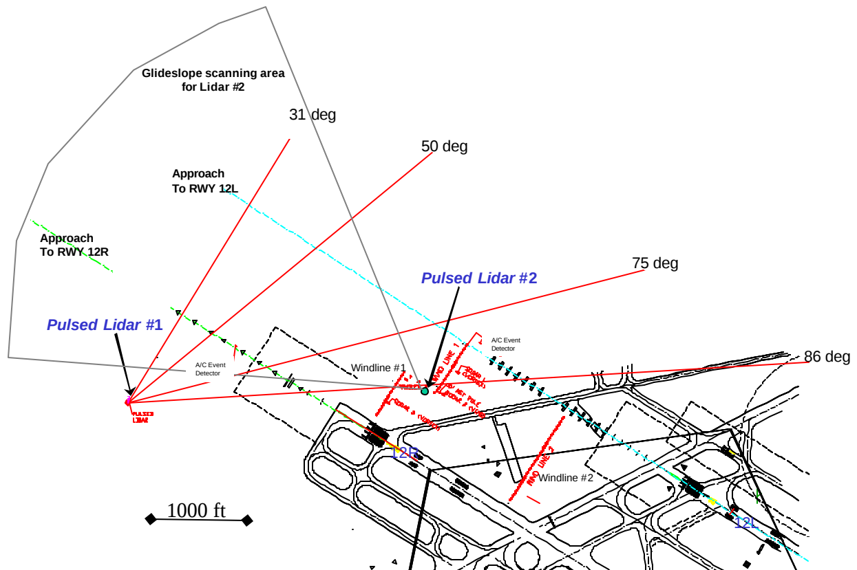
Figure 9 Instrument layout at St. Louis International Airport for wake and wind monitoring.
