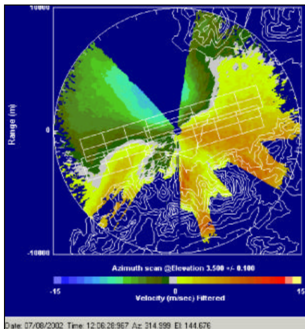
Figure 6 Sample PPI display of measured radial velocity with an overlay of the airport alerting area and nearby Lantau Island. Flow is out of the NNW.
