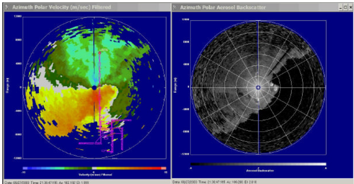
Figure 8 Sample PPI display of measured radial velocity (left) and aerosol backscatter (right) at DEN on 27 August 2003. The 2.0 degree elevation angle tilt is shown. The radial velocity display is color-coded with positive velocity defined away from the lidar. The front is also clearly visible in the aerosol backscatter display, extending along a line running from the southwest to the northeast and advancing toward the southeast.
